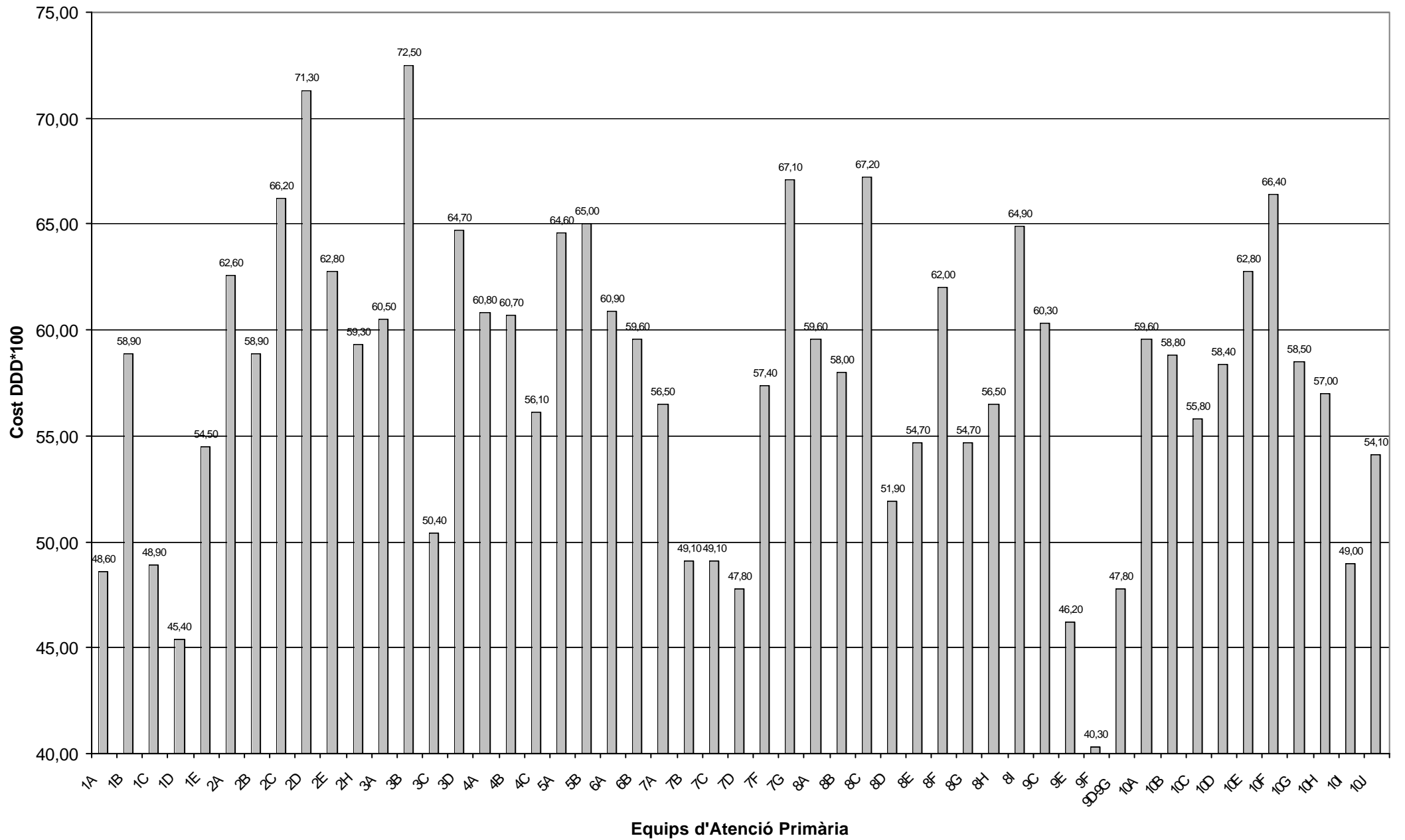
Figura 5.4. Cost AINE. 2002 Cost DDD*100
